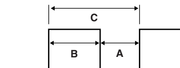
Fig. 1.17 Duty cycle
