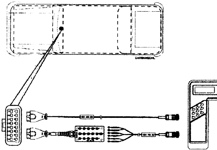
Fig. 4.5 The leads for the Bosch KTS 300 pocket system tester
