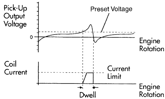
Low Speed Input/Output Waveforms
