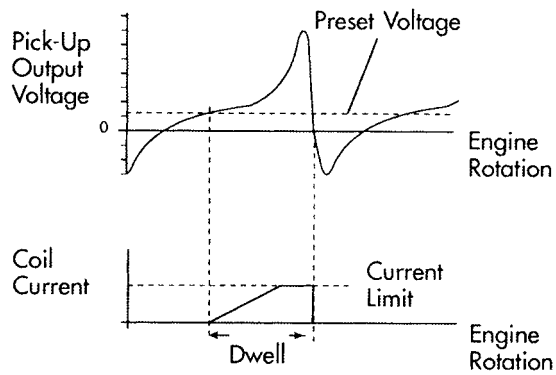
High Speed Input/Output Waveforms
