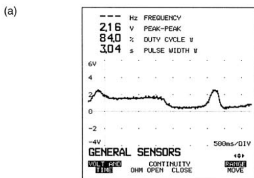
Fig. 7.28 Testing a manifold absolute pressure sensor
