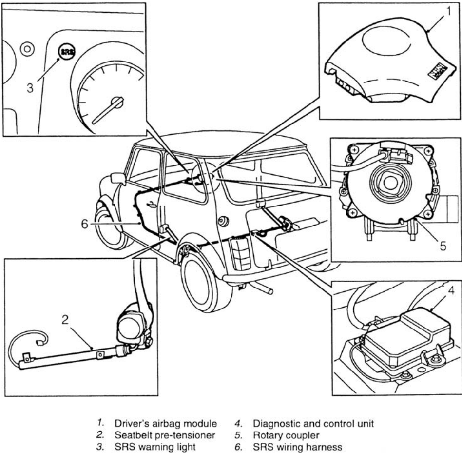
Fig. 8.20 The elements of a supplementary restraint system (Rover Mini)
