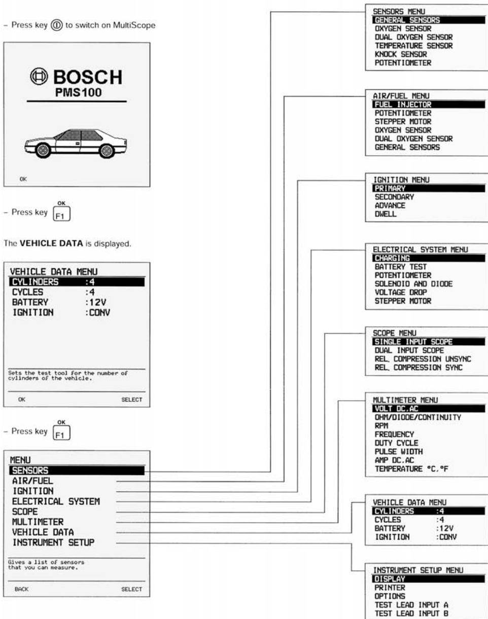
Fig. 4.13(b) An overview of available test functions from the MENU key of the Bosch PMS 100 portable oscilloscope
